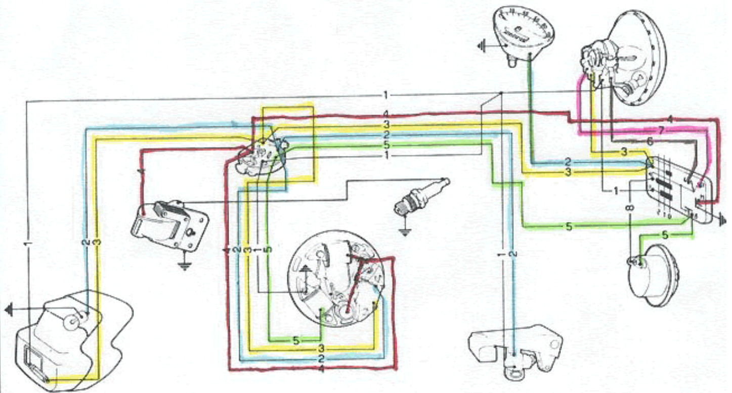
Wiring diagram — Vespa 150 Super VBC1 and 150 Sprint VLB1
